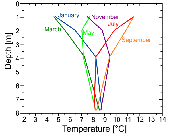
Figure 2: Measurement of ground temperature at the Royal Edinburgh Observatory, average values 1838-1854, after data from Everett (1860)
