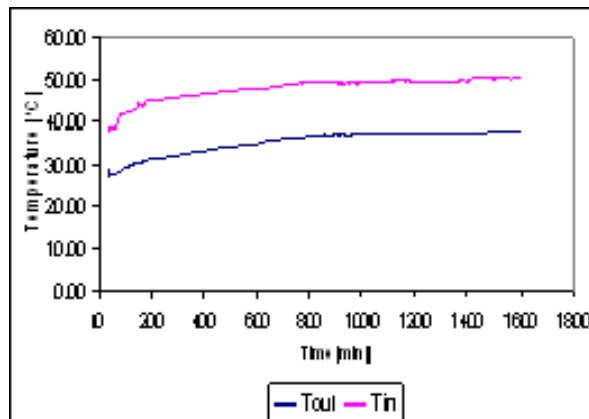
Figure 11: Evaluation Period of Double U BHE
