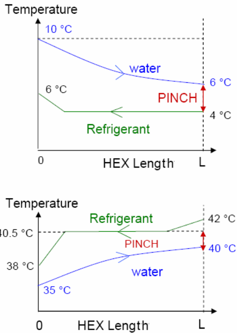
Figure 6: Temperature development in the GSHP, over the length of the heat exchanger for evaporator (above) and condenser (below)
