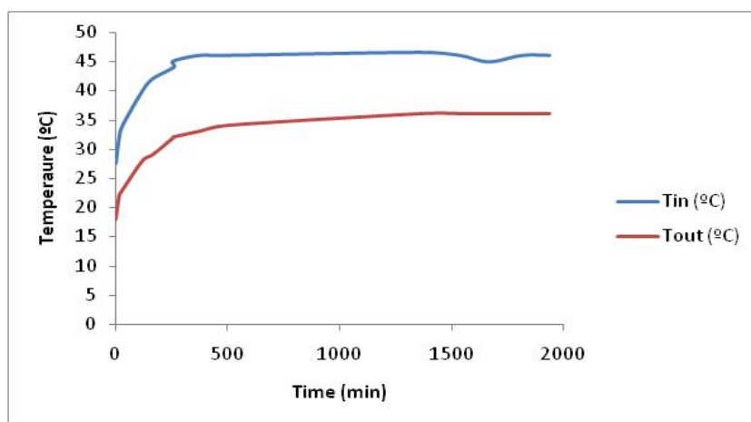
Figure 13: Evaluation Period of Coaxial BHE
